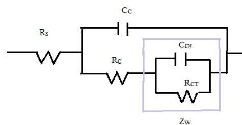
Randles circuit (a)
